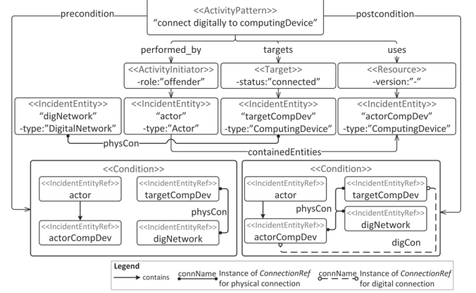
Fig. 11: “connect digitally to computingDevice” activity pattern.
