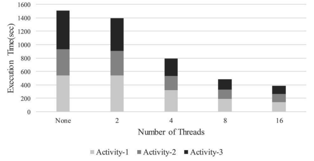
Fig. 18: Execution time of instantiating incident pattern activities using different number of threads in RC2 with LTS of size 10,000.
