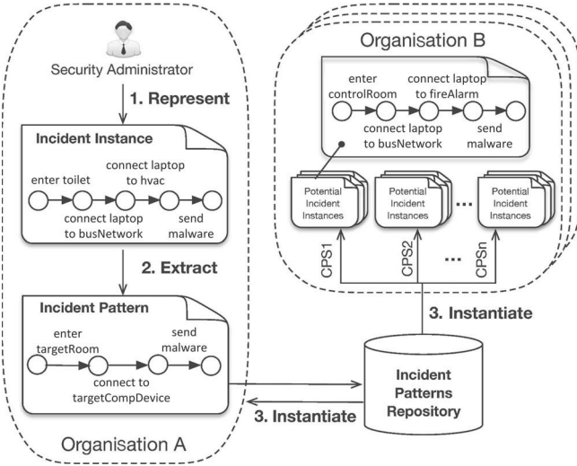
Fig. 2: Our approach for sharing incident knowledge.
