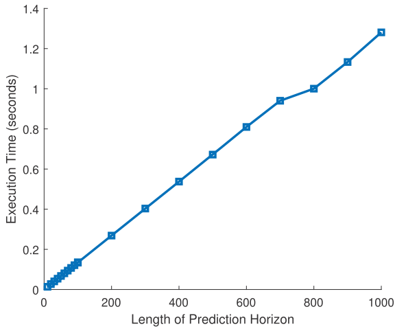
Fig. 8. Average execution time of the proposed scheme versus the number of steps for prediction.
