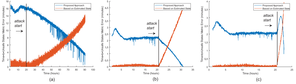
Fig. 7. Difference (error) between time-to-unsafe metric computed based on state estimate and based on the proposed algorithm versus the time-to-unsafe states based on the real state of the system. (a) Scenario 1. (b) Scenario 2. (c) Scenario 3.
