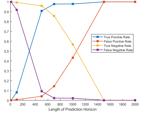
Fig. 2. True/false positive/negative rates as a function of the length of prediction horizon K .
