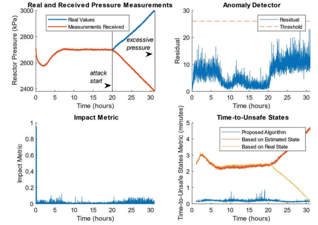
Fig. 5. Results from simulation Scenario 2.
