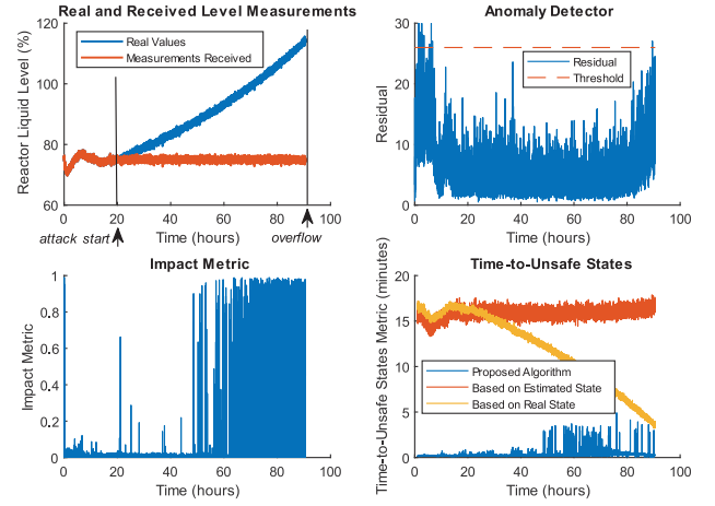
Fig. 4. Results from simulation Scenario 1.
